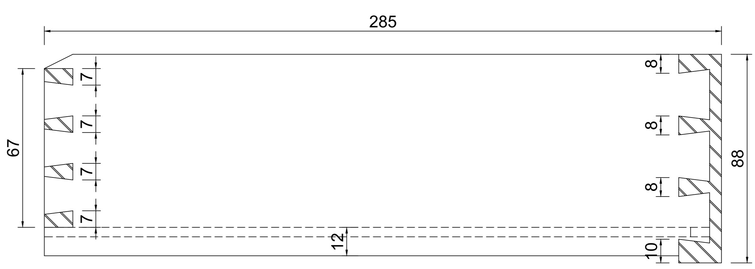
Drawer Detail
