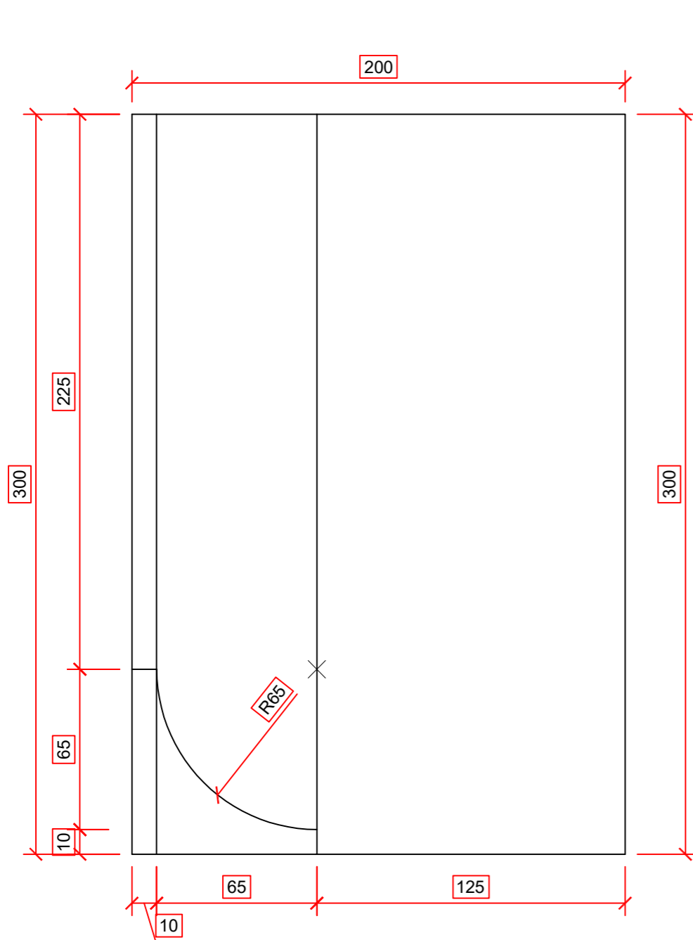
END VIEW
