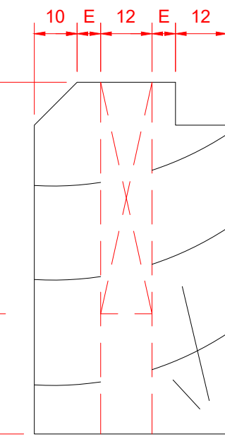
JOINT PROPORTIONS BOTTOM RAIL
